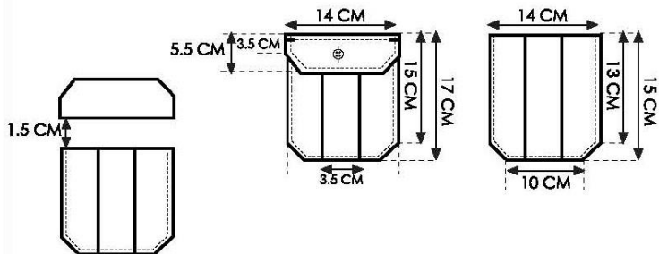
POCKET
